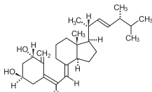
Figure 1: Chemical Structure of Doxercalciferol
